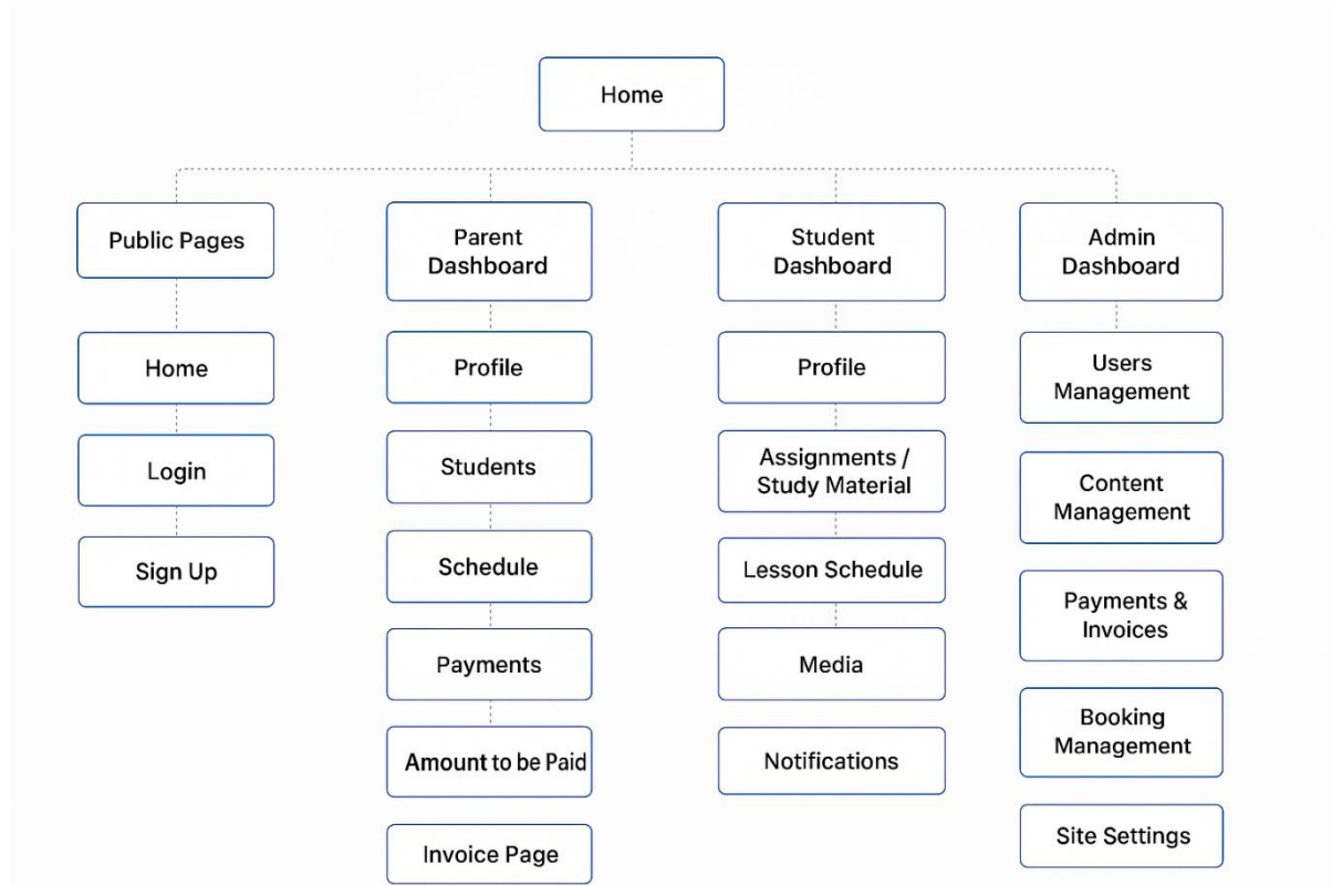
Tutoring Website Site Map Diagram
